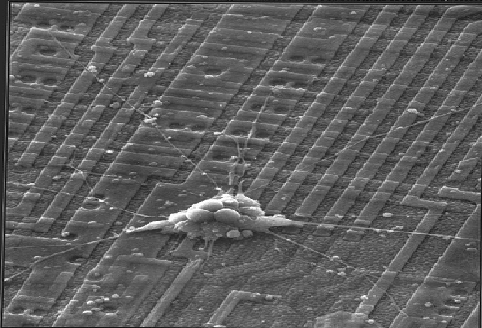
Scanning Electron Micrograph of a neuronal circuit grown in tissue culture on a Motorola 68000 microprocessor
